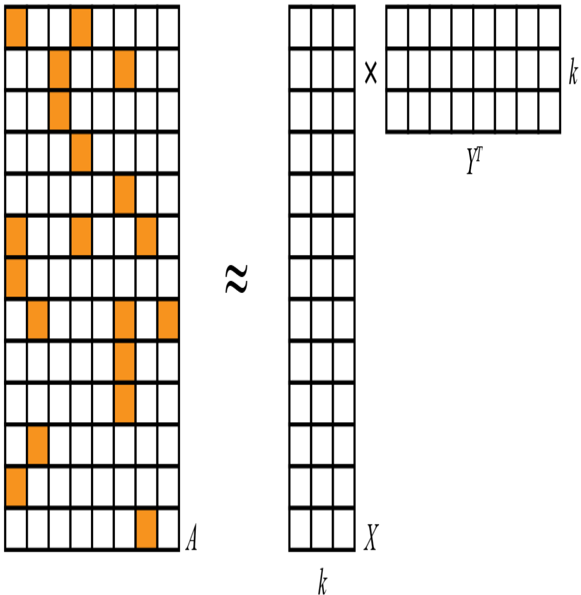
Figure 3-1. Matrix factorization
