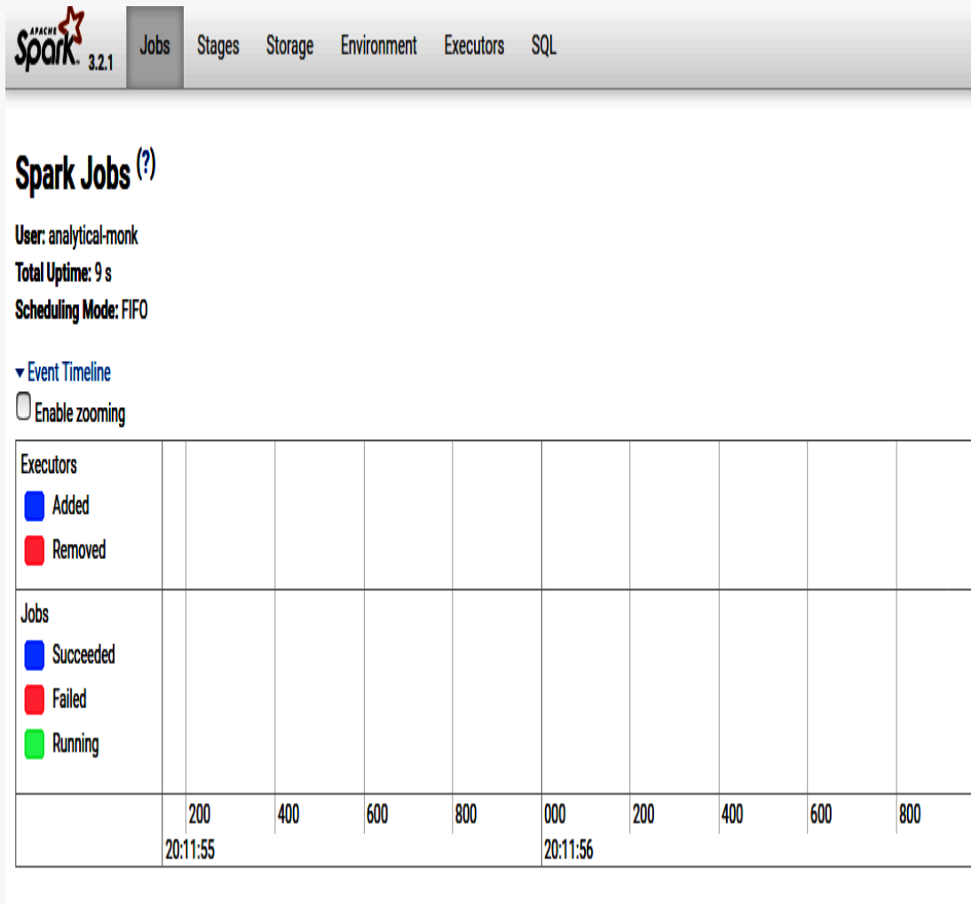
Figure 3-3. Spark UI
