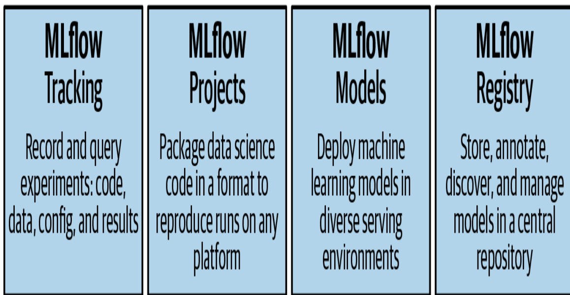
Figure 11-2. MLflow components
