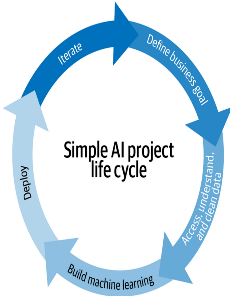
Figure 11-1. ML lifecycle
