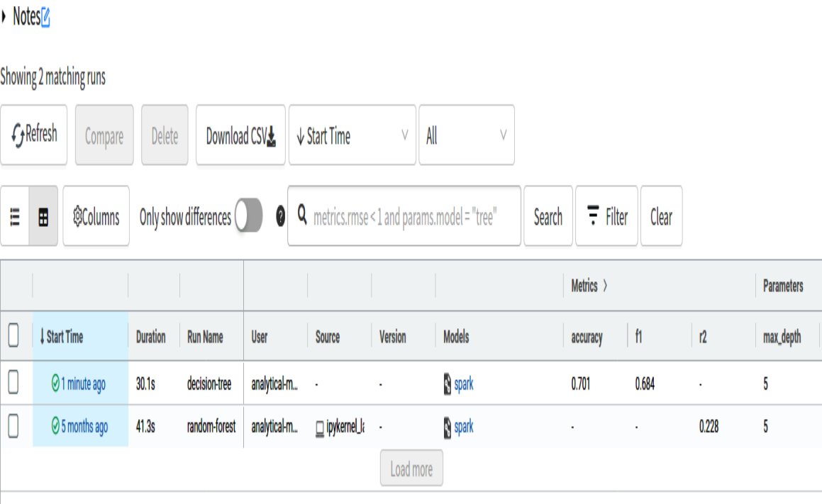
Figure 11-3. MLflow UI 1
