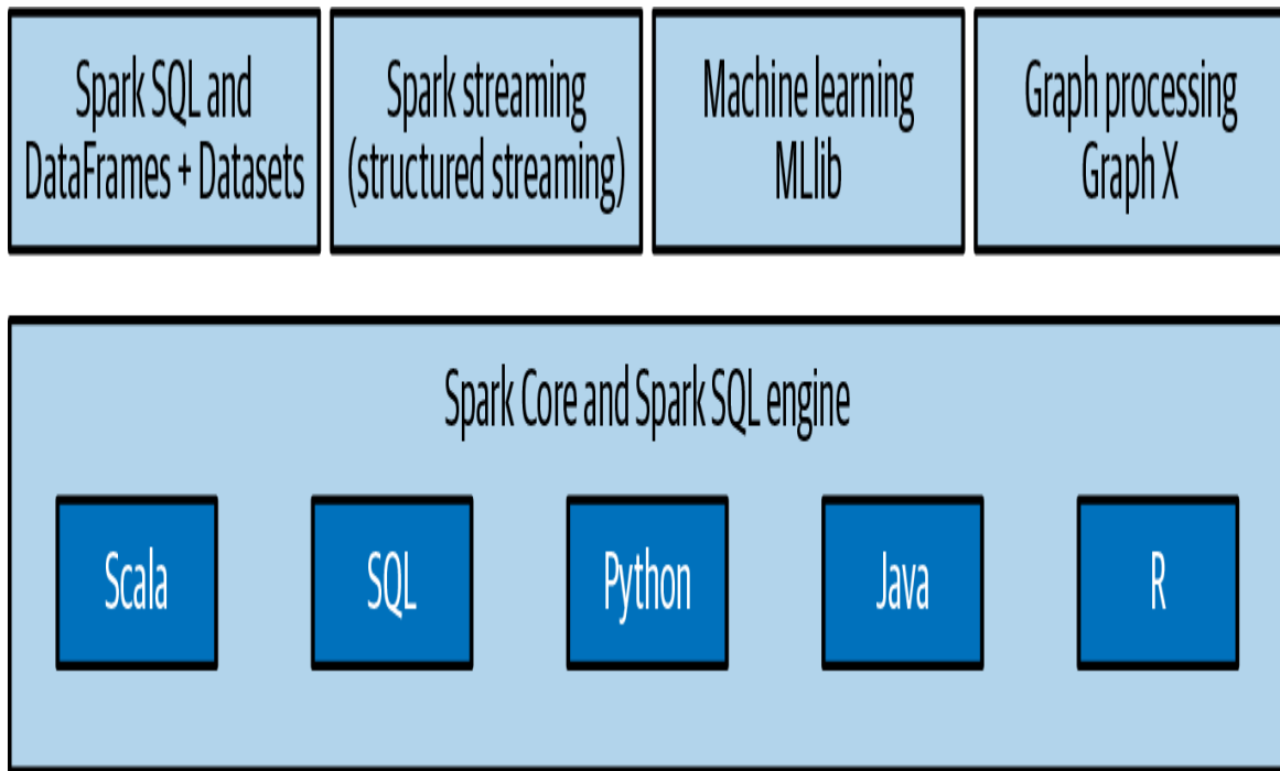
Figure 1-1. Apache Spark components
